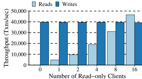
Figure 10: Backup’s read-only and read-write transaction throughput as the read-only load increases.
