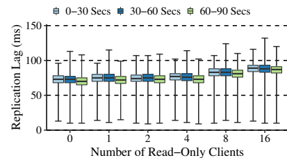
Figure 9: Replication lag of read-write transactions with increasing number of read-only clients.
