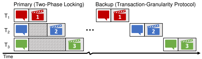
Figure 2: Primary (2PL) and backup (transaction-granularity protocol) executions when three users comment on the same video. Diagonal lines depict waiting for a lock.
