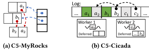
Figure 6: Scheduling and execution in each implementation. Refer to the accompanying text for details.
