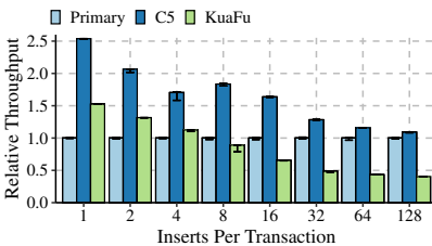
Figure 12: Primary and backup’s throughput on adversarial workload as inserts per transaction increases.
