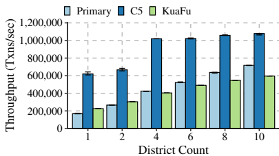
Figure 11: Primary and backup’s throughput on 50%-50% NewOrder-Payment with increasing districts.
