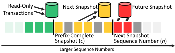
Figure 5: C5’s snapshotter. Writes in color (grey) have finished (not finished) executing.
