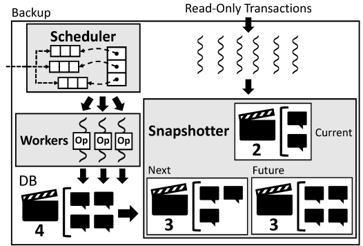
Figure 3: C5’s scheduler, workers, and snapshotter.
