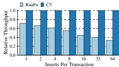
Figure 8: Backup’s throughput relative to primary’s on adversarial workload as inserts per transaction increases.
