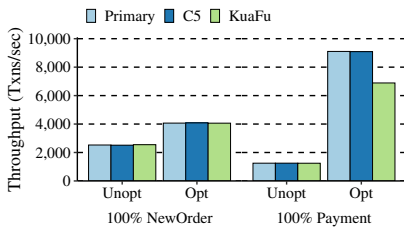
Figure 7: Throughput on 100% NewOrder and 100% Payment before and after optimization.
