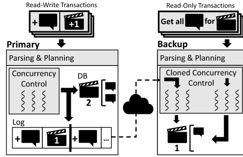
Figure 1: Transaction processing in primary-backup.
