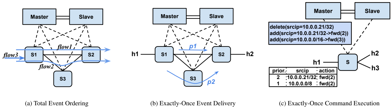
Figure 2: Examples demonstrating different correctness properties maintained by Ravana
