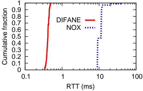
Figure 8: Delay comparison of DIFANE and NOX.
