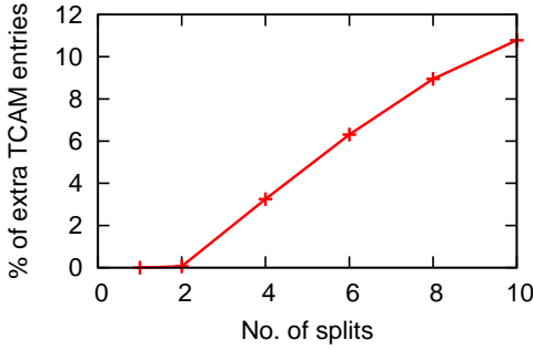
Figure 13: The overhead of rule partition.
