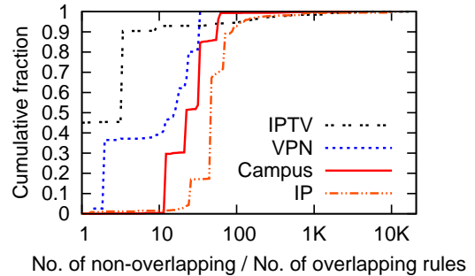
Figure 11: Comparison of overlapping and non-overlapping rules.
